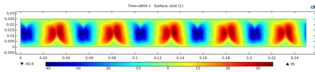
Figure 1: MHD natural convection
